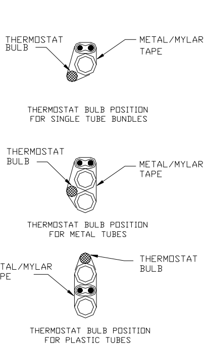
CORE CROSS-SECTION
